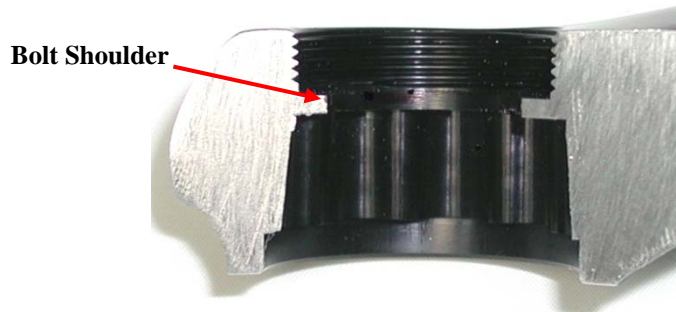
Non-Drive arm cross-section
